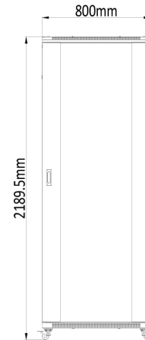
Vista frontal
