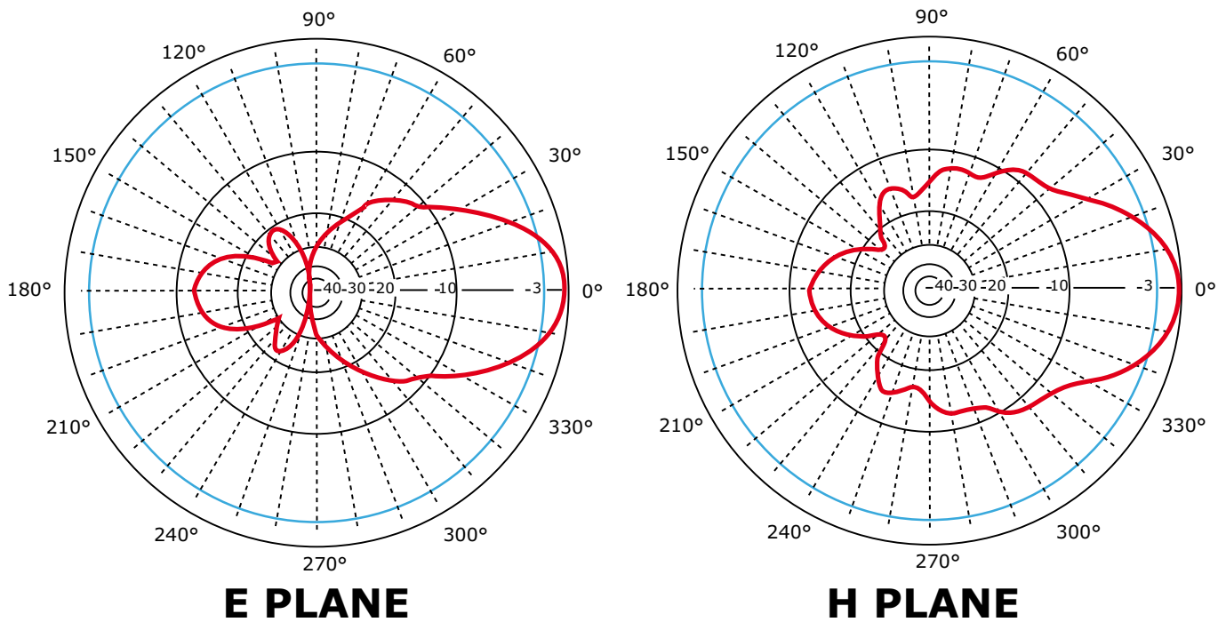
LP-YAGI2415XY 15 dBi 2.4 GHz YAGI Antennas
