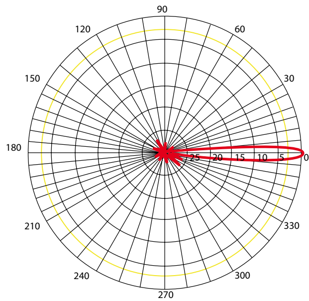
H PLANE
