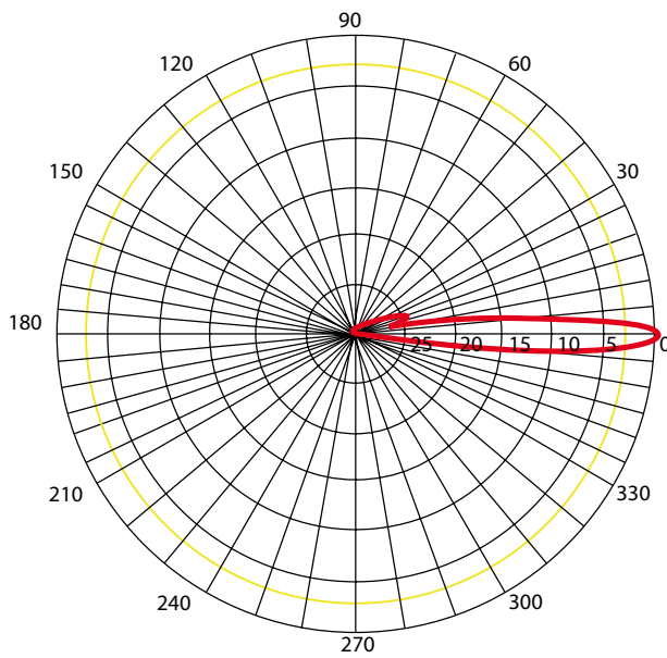
E PLANE
