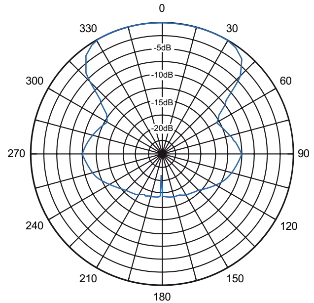
E Plane
