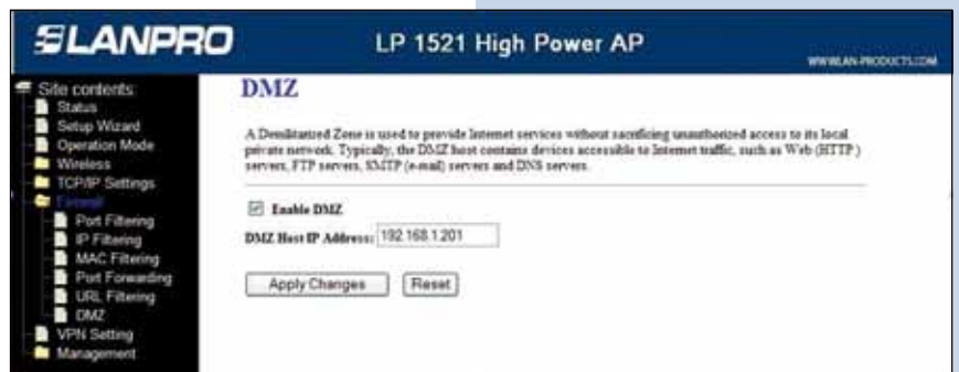
Screen snapshot – Firewall - DMZ Figure 32
