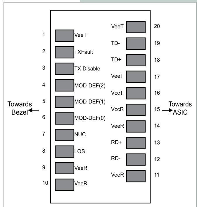
Figure 1. SFP to host connector pin assignments and descriptions
