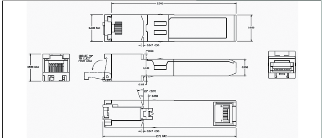
Figure 2. LP-OSFPT0X mechanical dimensions
