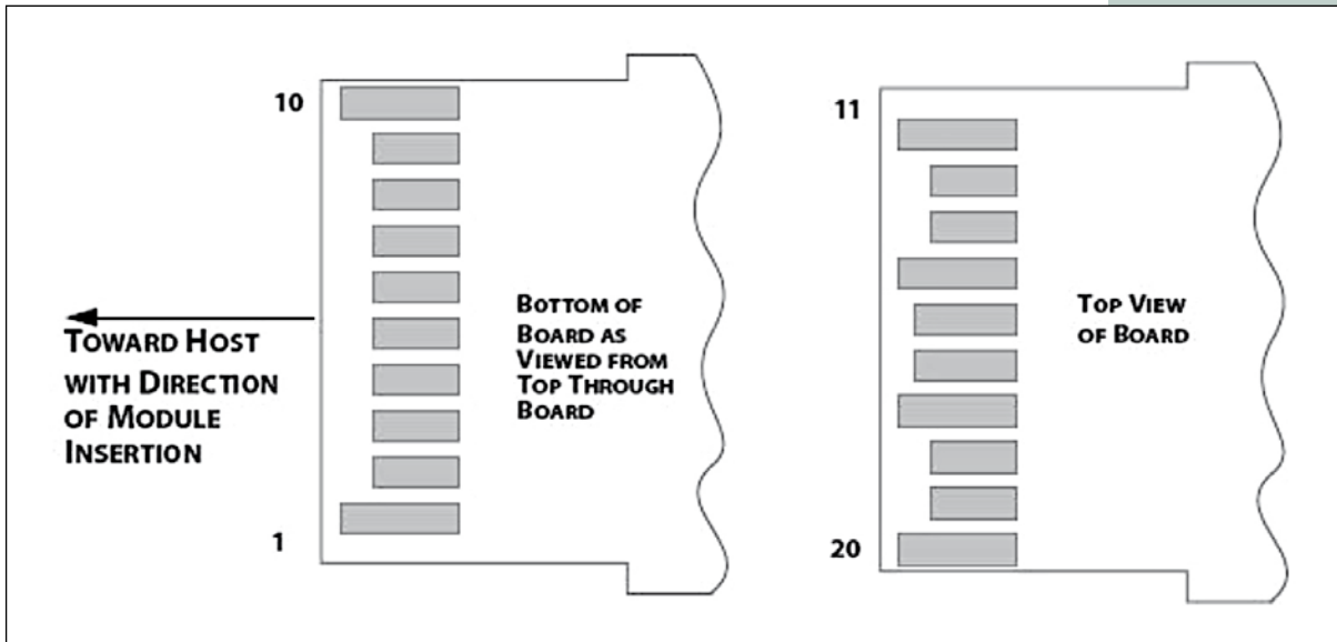
Figure 3: Module contact Assignment
