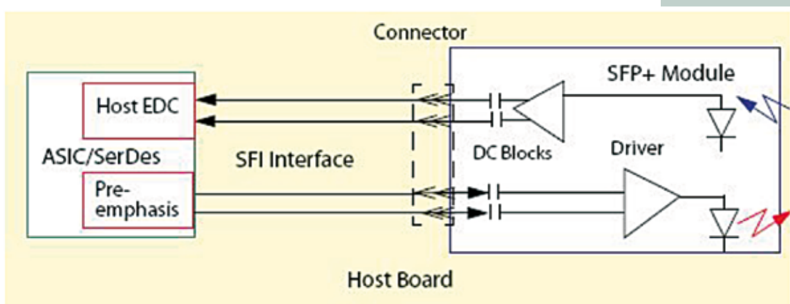
Figure 1: Interface to Host
