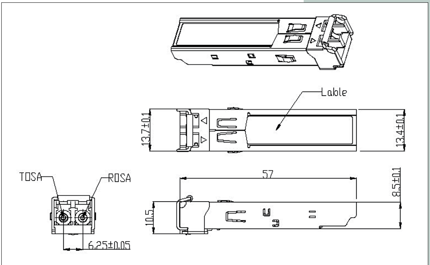
Key Mechanical Dimensions
